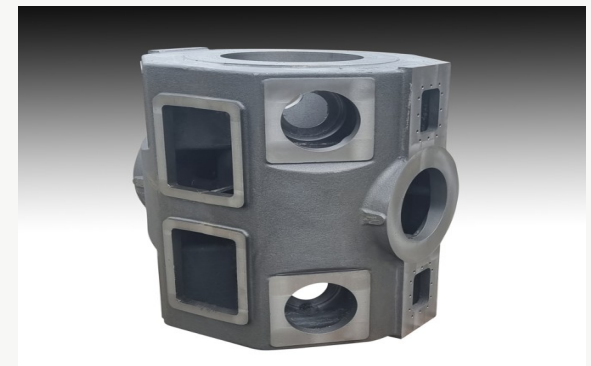
Cylinder · FCD450 (500Kg~4t)
